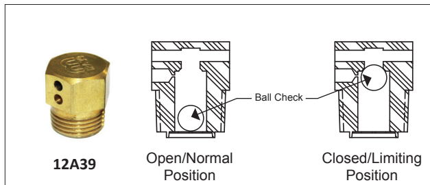
Figure 9: 12A39 Ball Check Cutaway
